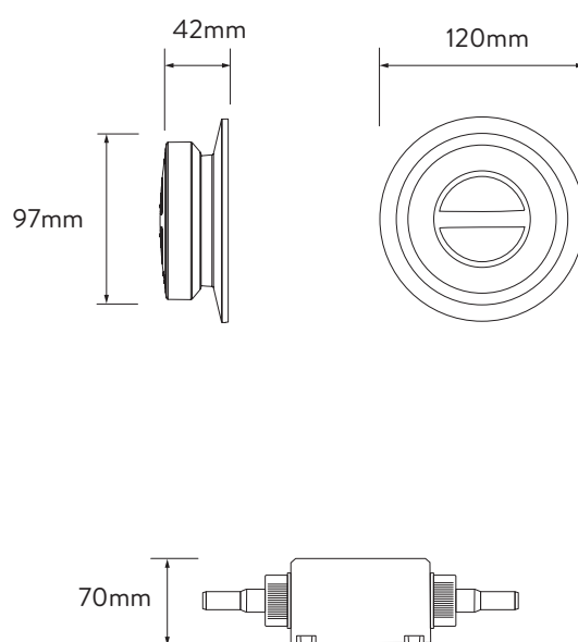
CONTROLLER
